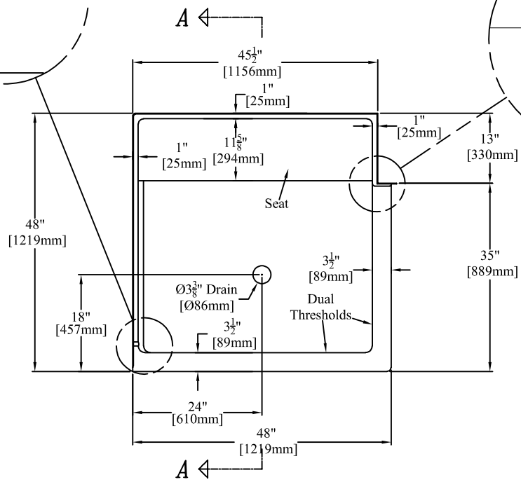
48" x 48" [1219mm x 1219mm] Corner Shower Pan w/ Dual 6" [152mm] Thresholds & Molded Seat on Back Wall
